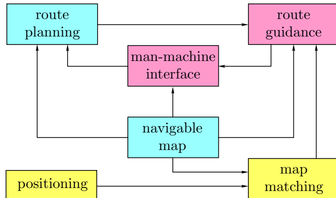
Figure 1: Components of a pedestrian navigation system
