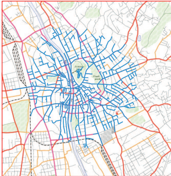
Figure 4: Search tree
